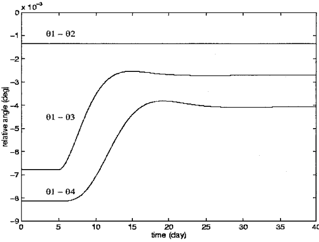
Fig. 7 Formation reconfiguration.
