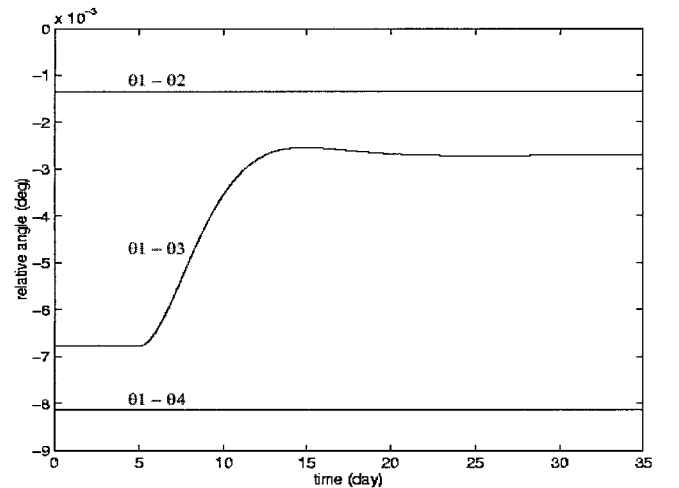
Fig. 4 Formation reconfiguration.
