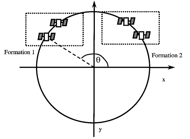
Fig. 2 In-plane formations in a circular orbit.
