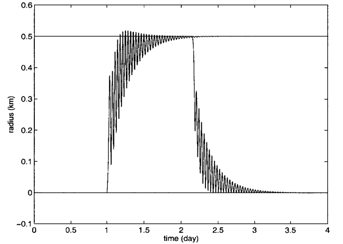
Fig. 13 Radius r_3 - 1 and r_4 - 1 .
