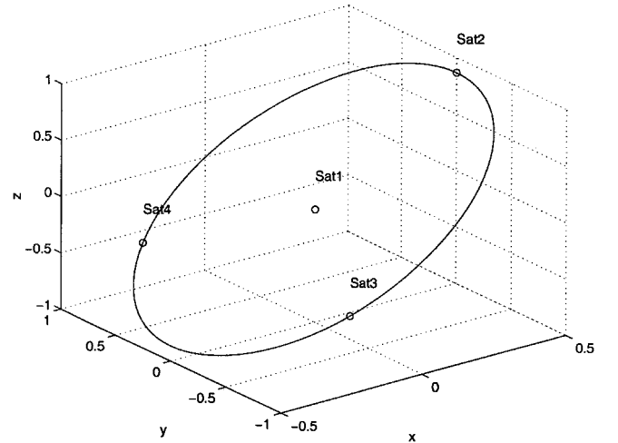
Fig. 9 Path of three satellites relative to sat1 in moving frame.
