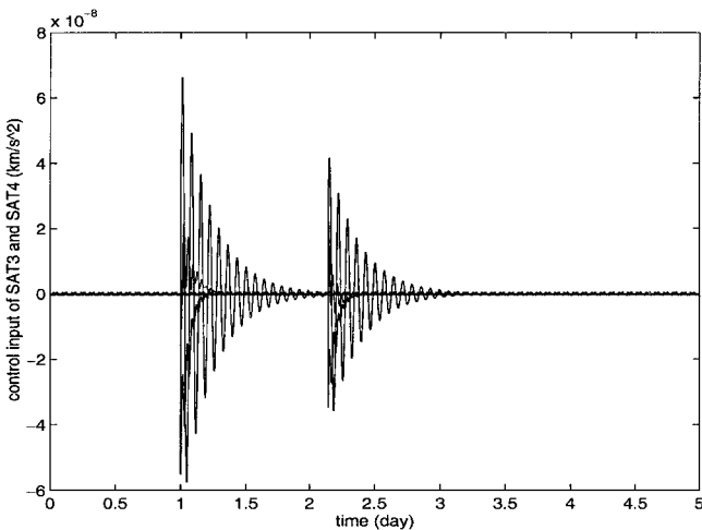
Fig. 16 Control inputs.
